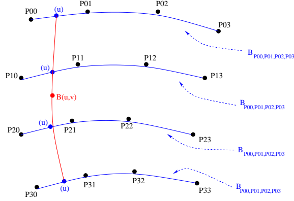
Figure 1: Recipe for a B-spline patch.
